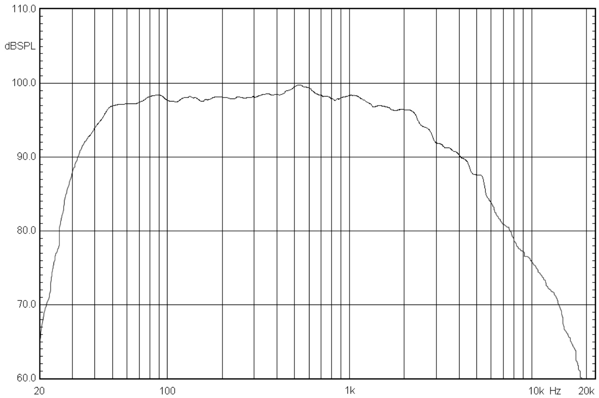
Void Acoustics : Mycro Bass - Active Input : 1w/1m
