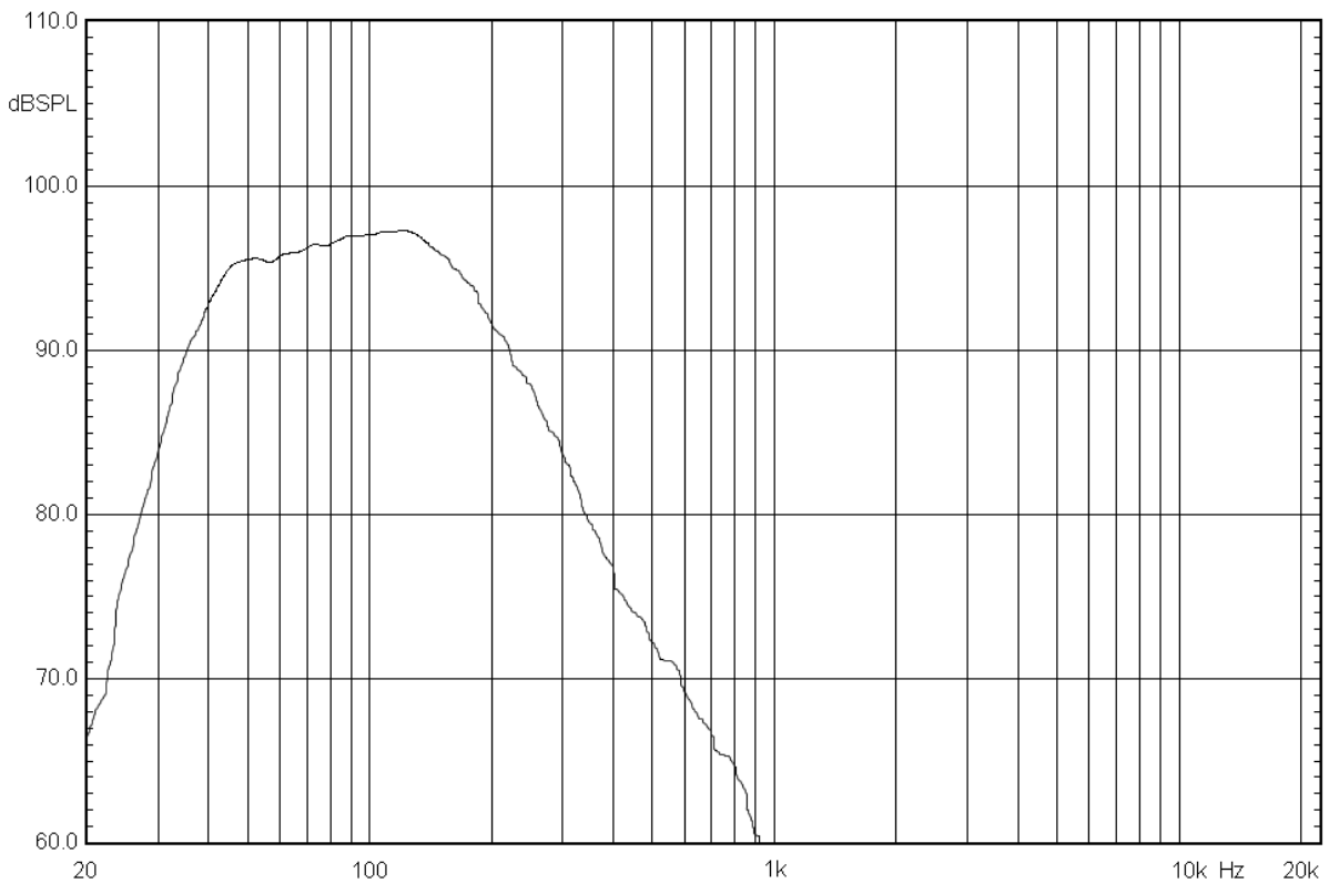
Void Acoustics : Mycro Bass - Passive Input : 1w/1m
